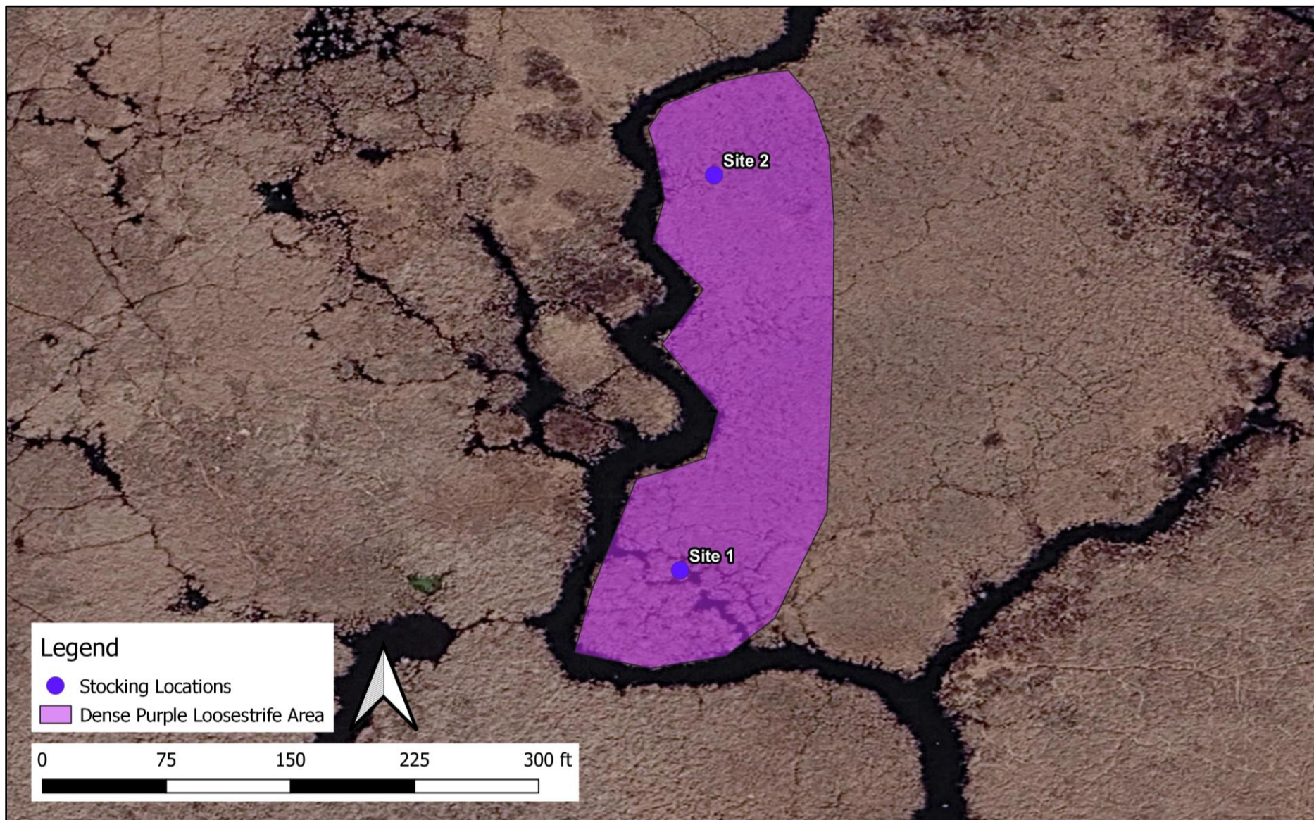
Figure 1. Aerial satellite imagery of purple loosestrife area and purple loosestrife biocontrol pot placement locations. Two stocking sites with clusters of four pots inoculated with Gallerucella sp. beetles.
